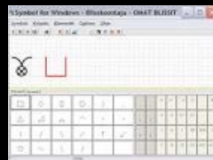
Bliss-Symbol Software
